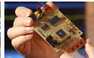
'Smart' wireless sensing device for structural health monitoring and control.
