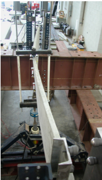
Lateral stability tests of reinforced and prestressed concrete beams.
