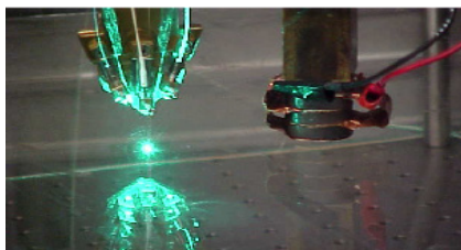
Fiber optic laser interferometer for structural damage detection.
